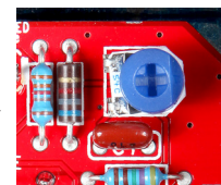
Treble Boost Variable Resistor Clockwise = More Counter-Clockwise = Less
